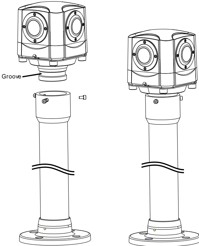
Figure 2-4 Install with column
