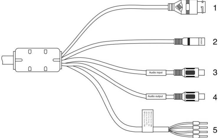
Figure 1-2 Multi-connector combination cable
