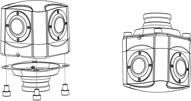
Figure 2-5 Fix the mounting bracket
