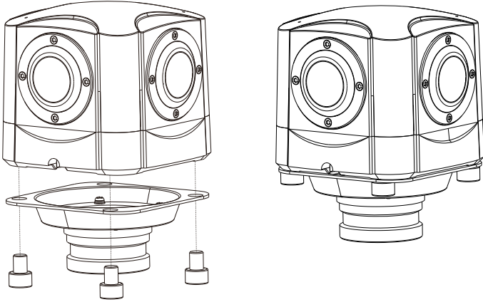
Figure 2-3 Fix the mounting bracket
