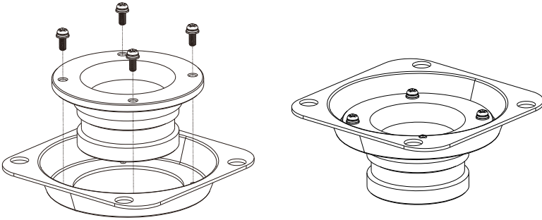
Figure 2-2 Dimension of bracket
