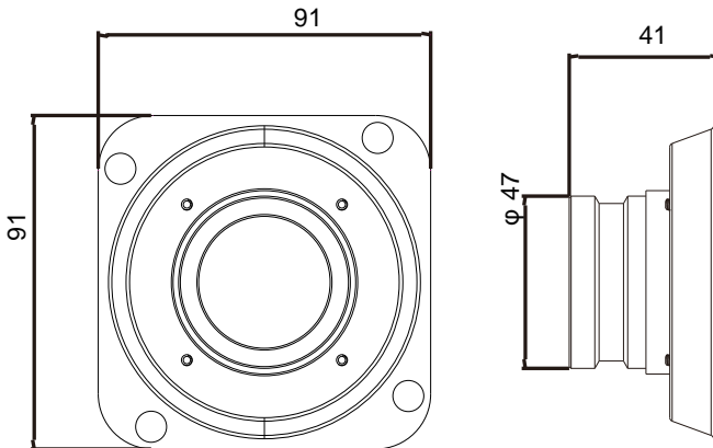
Figure 2-2 Dimension of bracket
